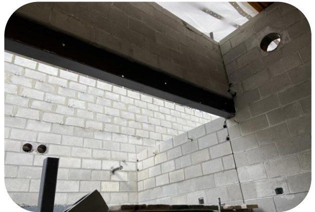
Steel beam header at gear room looking west to Line 5. Holes drilled in beam for ledger installation per structural engineer direction
