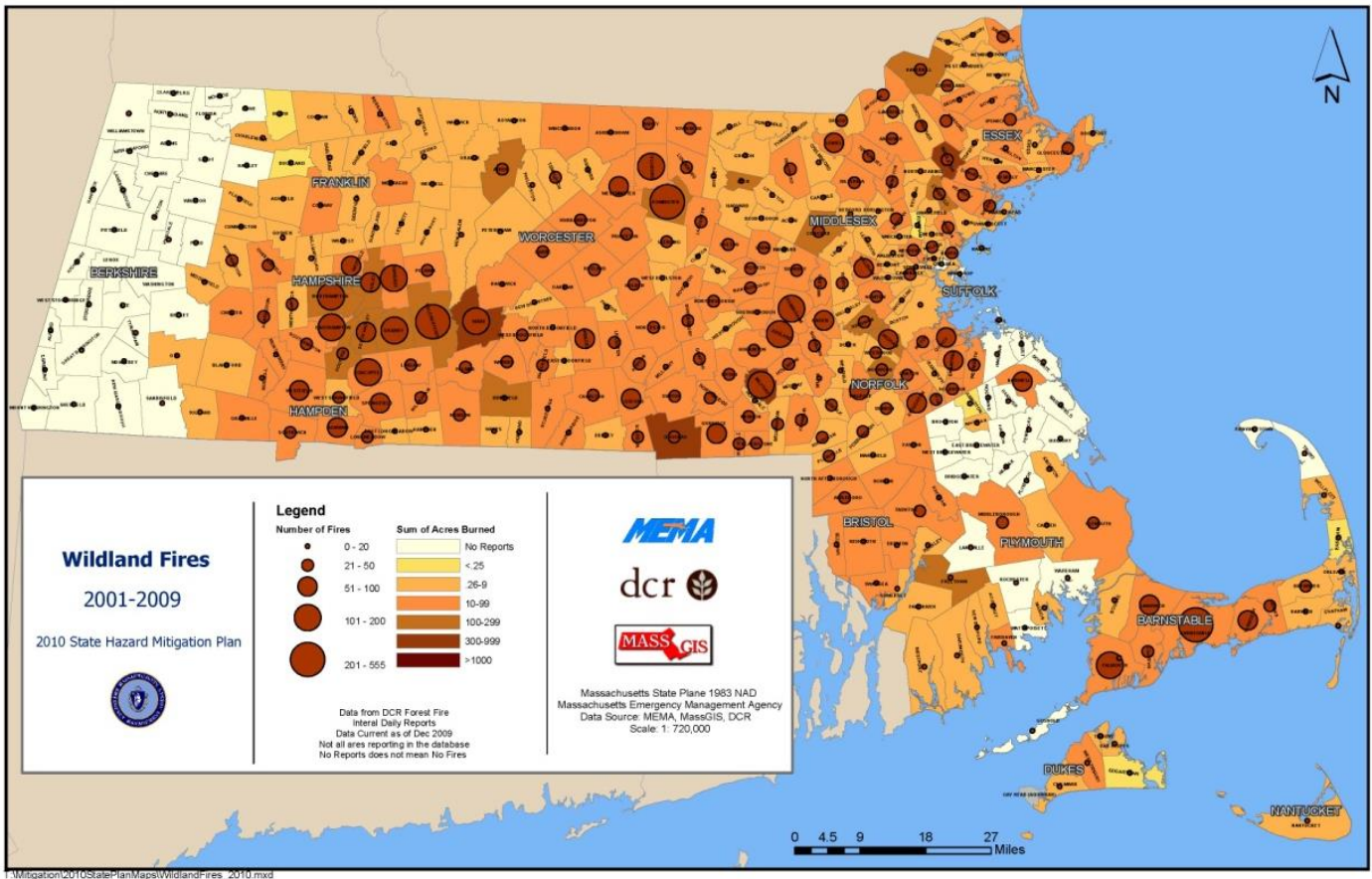
Figure 3: Massachusetts Wildfires, 2001 to 2009
