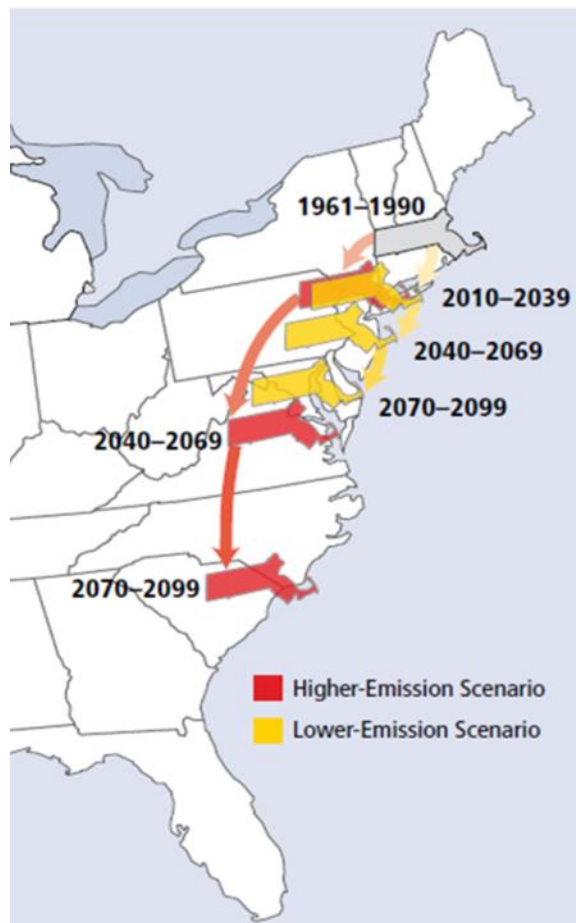
Figure 8 Mass. Extreme Heat Scenarios
