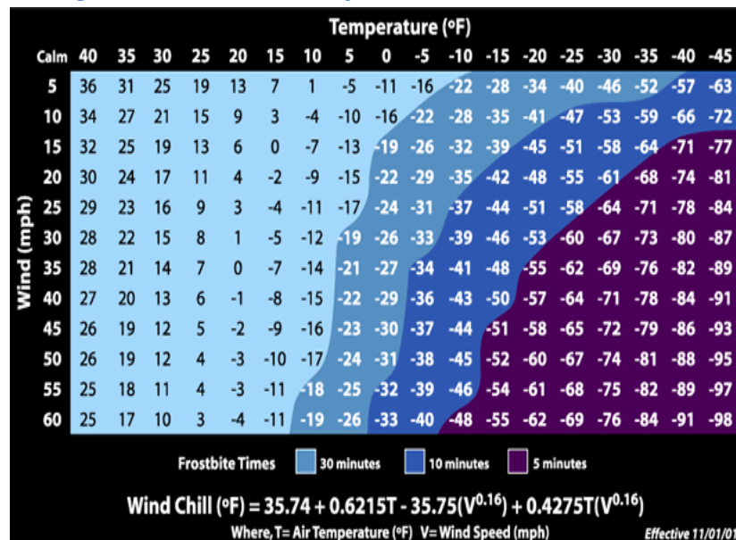
Figure 4: Wind Chill Temperature Index and Frostbit Risk
